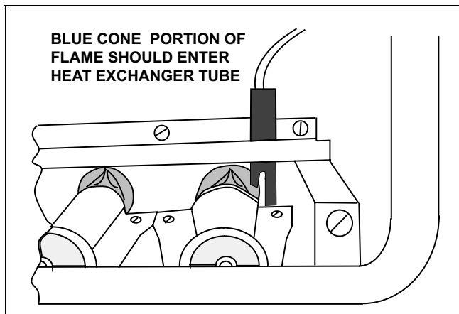
FIGURE 1: Proper Burner Flame Appearance
