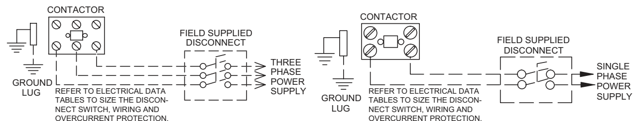
FIGURE 2 - TYPICAL FIELD WIRING DIAGRAM
