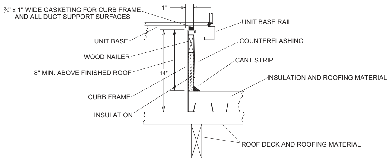
FIGURE 8 - ROOF CURB APPLICATION
