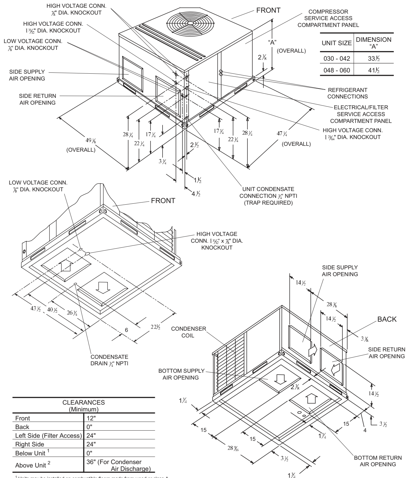
FIGURE 3 - UNIT DIMENSIONS
