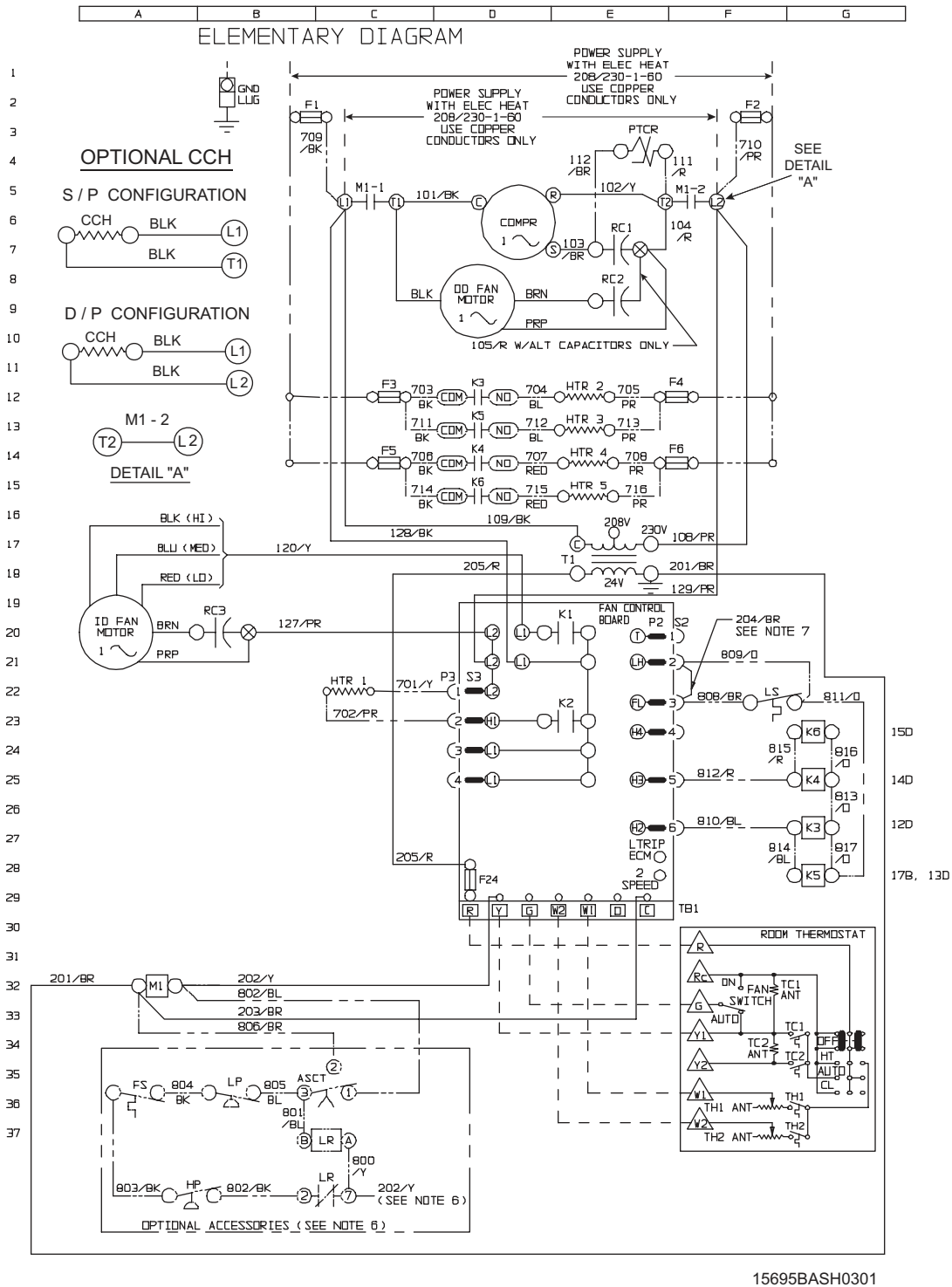
FIGURE 9 - TYPICAL WIRING DIAGRAM (208/230-1-60 POWER SUPPLY) DEB MODELS
