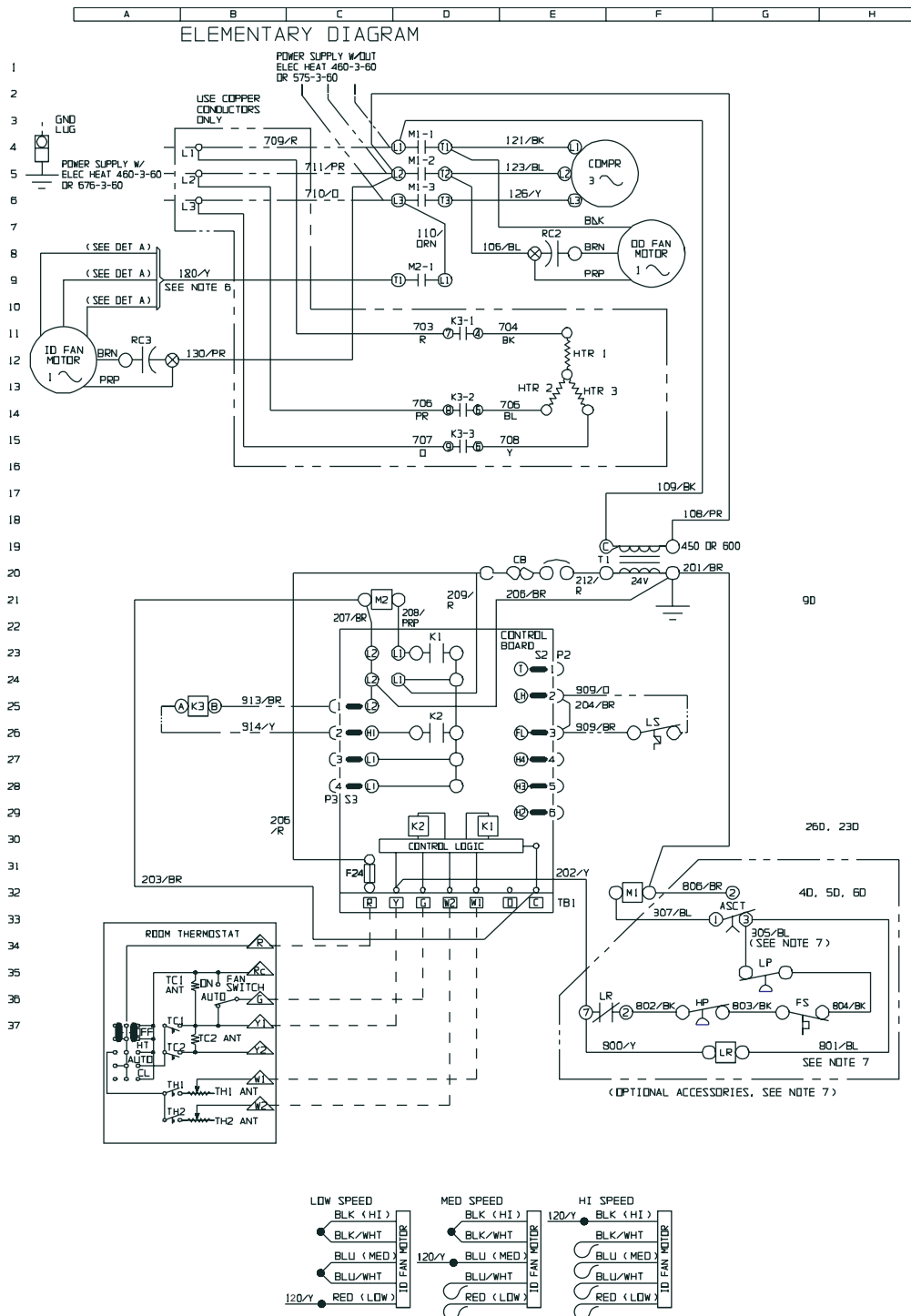
FIGURE 11 -TYPICAL WIRING DIAGRAM (460-3-60 AND 575-3-60 POWER SUPPLY) DEB MODELS
